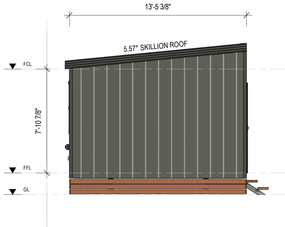
4 LEFT ELEVATION (4) A103 1 : 50
