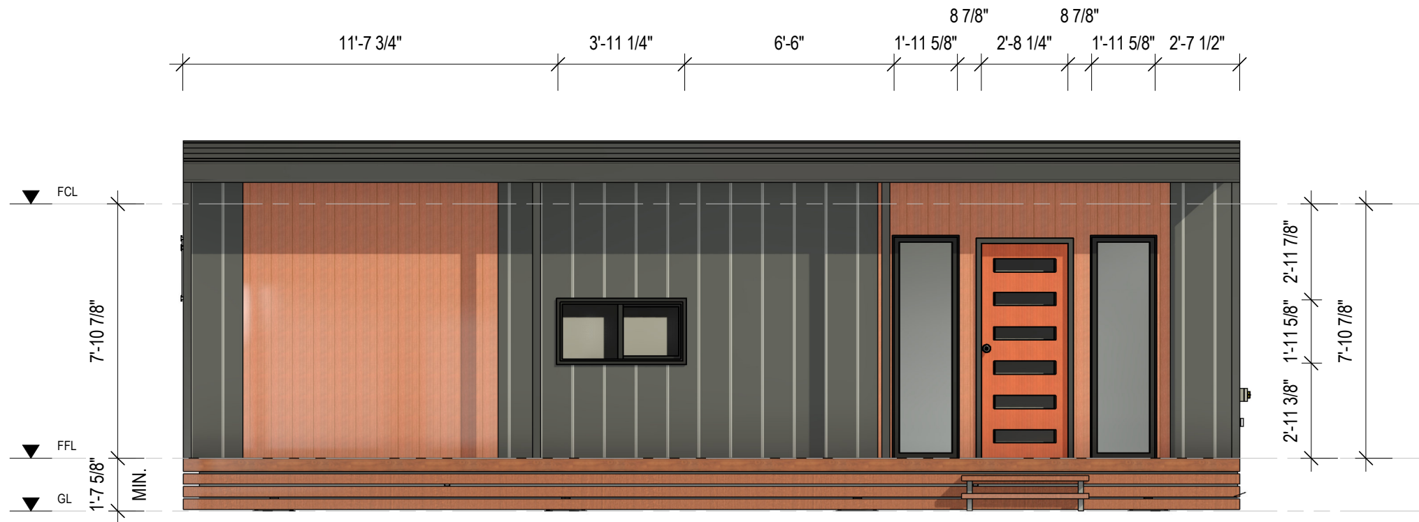
1 FRONT ELEVATION (1) A102 1 : 50
