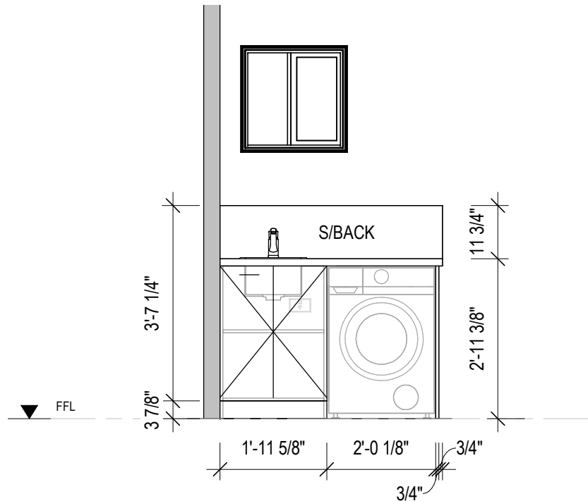
2 LAUNDRY ELEVATION A105 1 : 30
